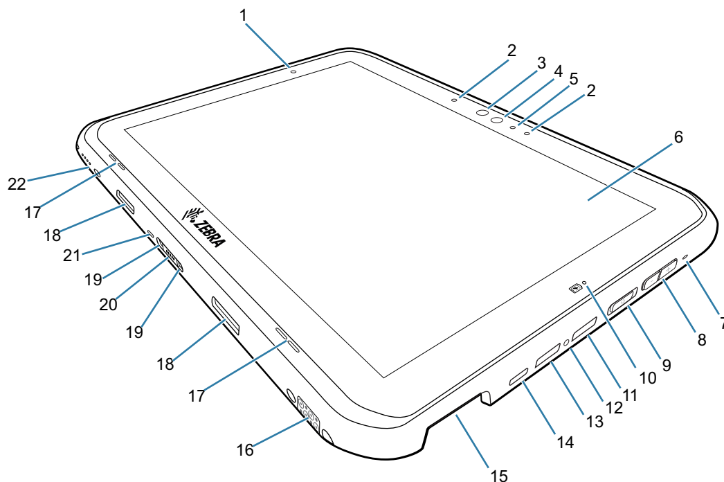
Figure 1 Front View
